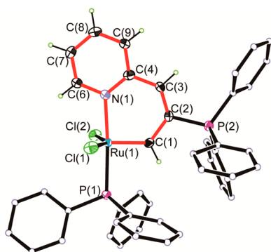
Figure 3. Molecular structure for the cation of 5 (ellipsoids at the 50% probability level). Counteranion and hydrogen atoms in \text{PPh}_3 are omitted for clarity. Selected bond lengths [ \text{\AA} ] and angles [deg]: Ru(1)–C(1) 1.834(3), C(1)–C(2) 1.458(4), C(2)–C(3) 1.336(5), C(3)–C(4) 1.449(5), N(1)–C(4) 1.360(4), Ru(1)–N(1) 2.117(3), N(1)–Ru(1)–C(1) 92.62(12), Ru(1)–C(1)–C(2) 125.8(2), C(1)–C(2)–C(3) 127.5(3), C(2)–C(3)–C(4) 127.6(3), C(3)–C(4)–N(1) 119.5(3), C(4)–N(1)–Ru(1) 126.9(2), Cl(1)–Ru(1)–Cl(2) 148.08(3), Cl(1)–Ru(1)–C(1) 107.96(10), Cl(2)–Ru(1)–C(1) 103.81(10).
